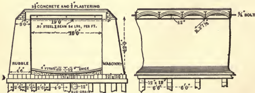
FIG. 10. CANAL STREET SEWER; ST. PAUL, MINN.
